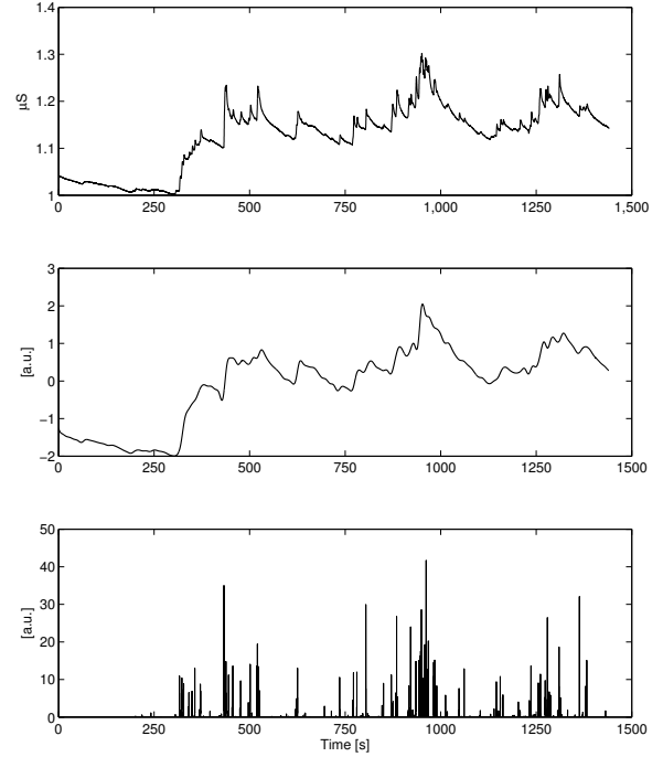
Fig. 1. Application of the cvxEDA decomposition procedure to the SC signal recorded during the affective sound stimulation for a representative subject. (Top) Raw SC signal, (Middle) Estimated slow tonic component t , (Bottom) Estimated sparse phasic driver component p .
